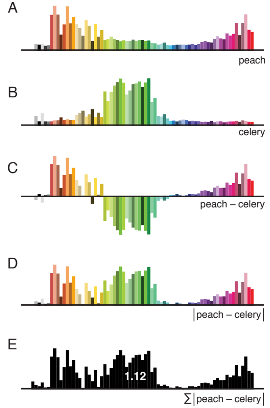
Figure S.4: The color-concept distributions for peach (A) and celery (B), the difference (C) between those two distributions, the absolute value (D) of that difference, and the sum of the elements in the result (E). Half of the final number would be the TV computed for peach and celery.
